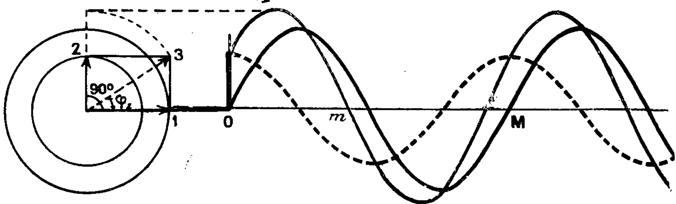
Fig. G 2 Y = a \sin \left( \omega t + \frac{\pi}{2} \right) + b \sin \omega t
