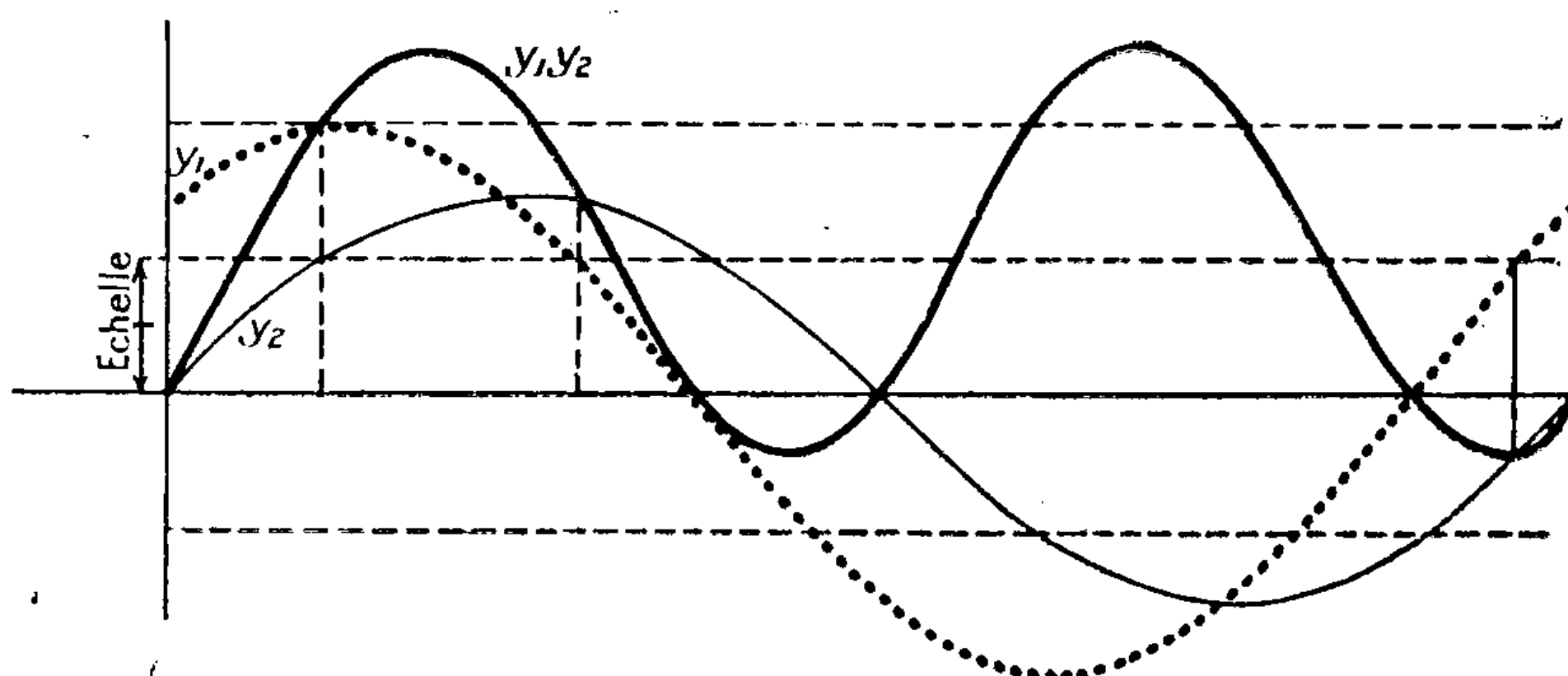
Fig. O 2 y_1 y_2 = 2 \sin \left( \omega t + \frac{\pi}{4} \right) 1,5 \sin \omega t .
